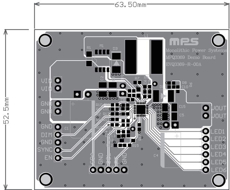
Figure 1: Top Layer
