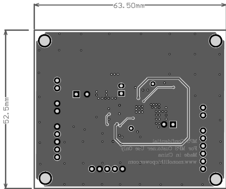
Figure 2: Bottom Layer
