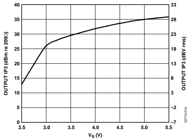
Figure 14. Output Third-Order Intercept vs. Supply Voltage at 70 MHz, V_{GAIN} = 500\text{ mV}
