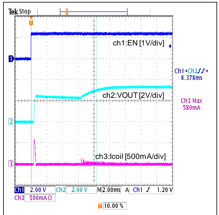
Figure 24. Start-up Waveform (VIN=2.4V, 3.3KΩ resistive load, MODE=H:Auto-PFM/PWM)
