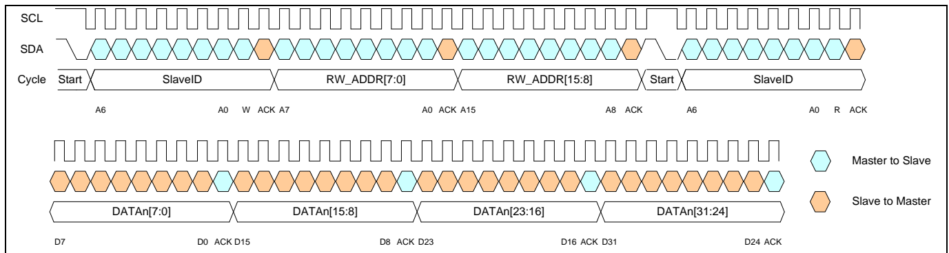
Figure 10. Read Access
