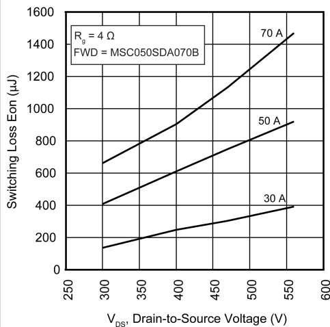
Figure 15 • Switching Energy Eon vs. V_{DS} and I_D
