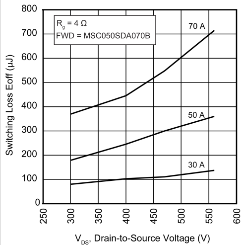
Figure 16 • Switching Energy Eoff vs. V_{DS} and I_D
