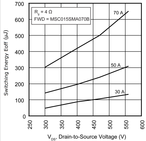
Figure 12 • Switching Energy Eoff vs. V_{DS} and I_D
