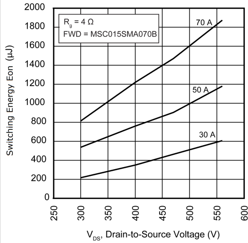
Figure 11 • Switching Energy Eon vs. V_{DS} and I_D
