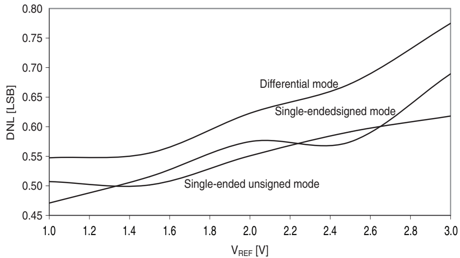
Figure 38-38. DNL error vs. external V_{REF} . T = 25^{\circ}\text{C} , V_{CC} = 3.6\text{V} , external reference.
