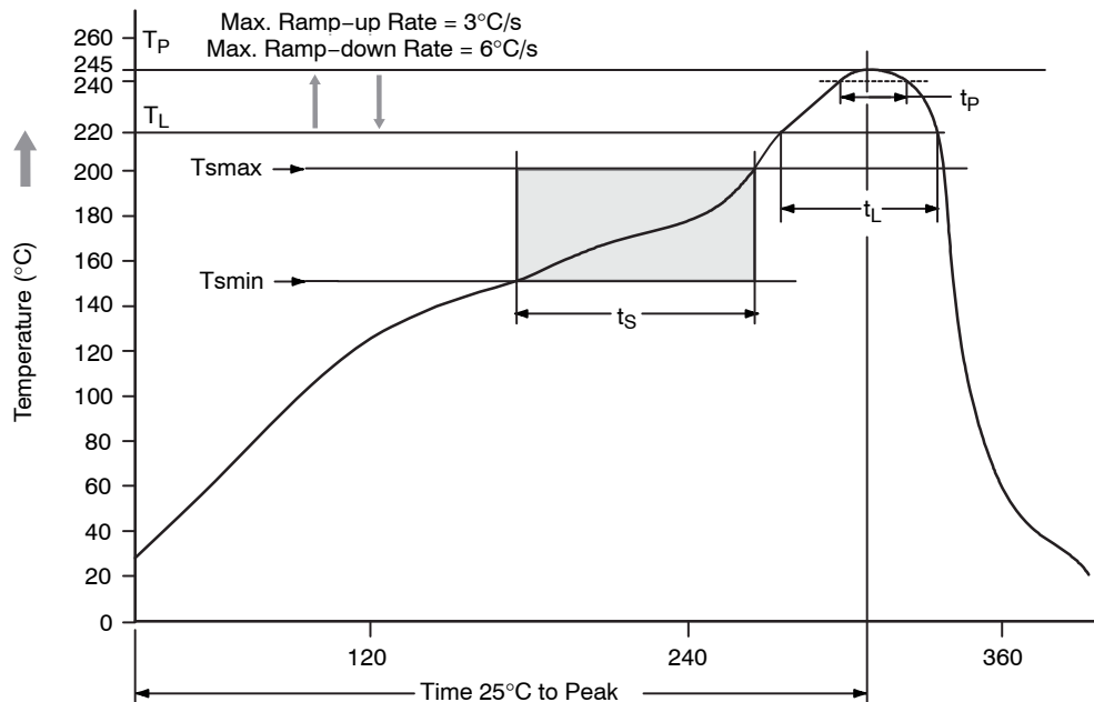
Figure 15. Reflow Profile
