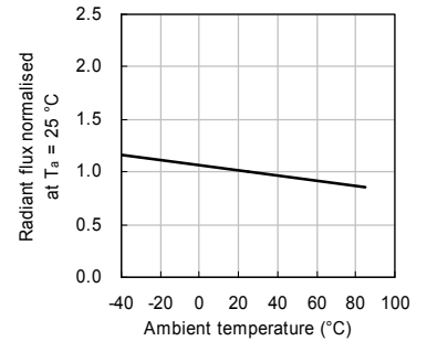
Radiant Flux vs. Ambient Temperature
