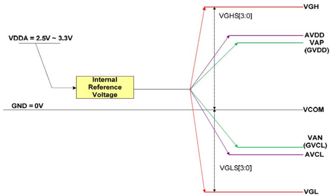
Fig.2 Voltage Generation
