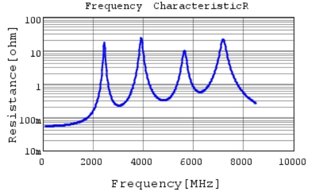
GQM1875C2E560GB12 R DC0V, 25degC
