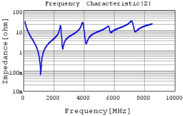
GQM1875C2E560GB12 |Z| DC0V, 25degC
