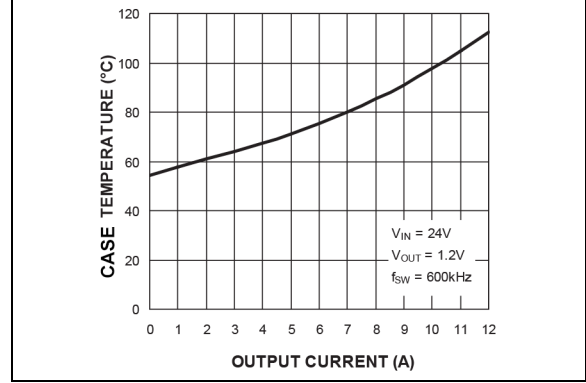
FIGURE 2-42: Case Temperature* ( V_{IN} = 24V ) vs. Output Current.
