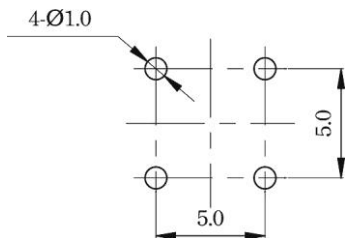
Mounting
