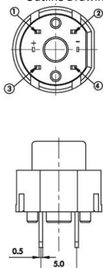
Outline Drawing
