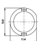
Outline Drawing
