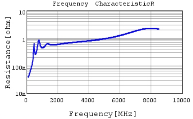
GCM1885C1H821JA16 R DC0V, 25degC
