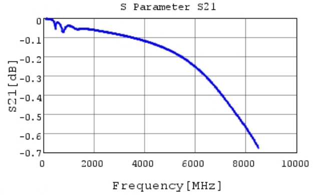
GCM1885C1H821JA16 S21 DCOV, 25degC
