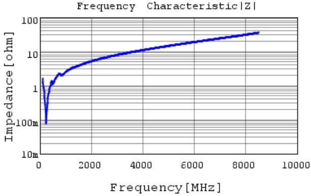
GCM1885C1H821JA16 |Z| DC0V, 25degC
