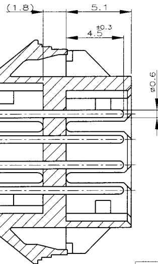
SECT. A-A
