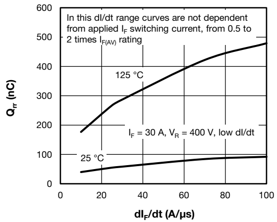
Fig. 11 - Typical Reverse Recovery Charge vs. di/dt , Per Leg
