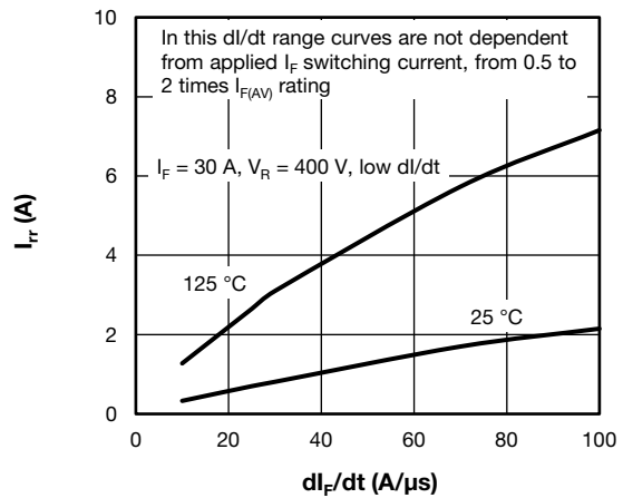
Fig. 12 - Typical Reverse Recovery Current vs. di/dt , Per Leg
