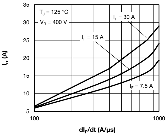
Fig. 9 - Typical Reverse Recovery Current vs. di/dt , Per Leg
