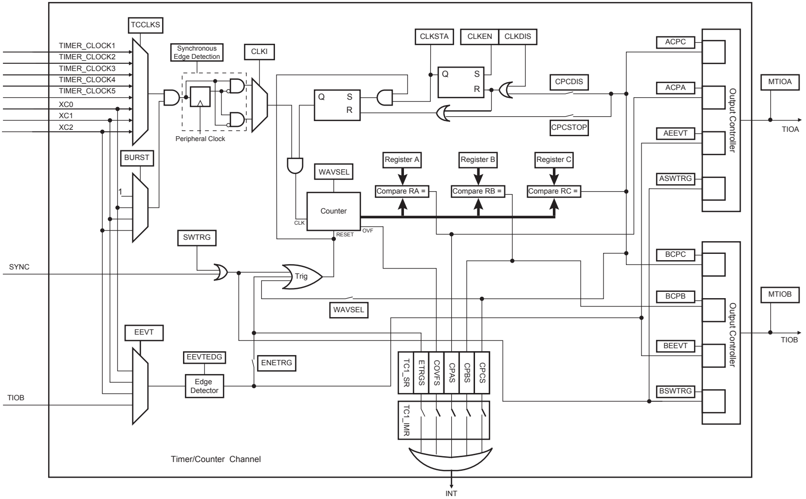
Figure 35-6: Waveform Mode
