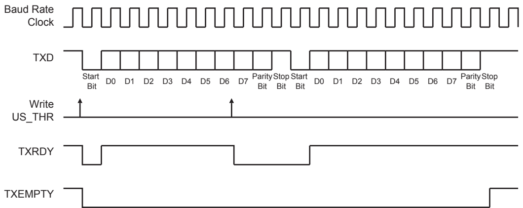
Figure 38-6: Transmitter Status
