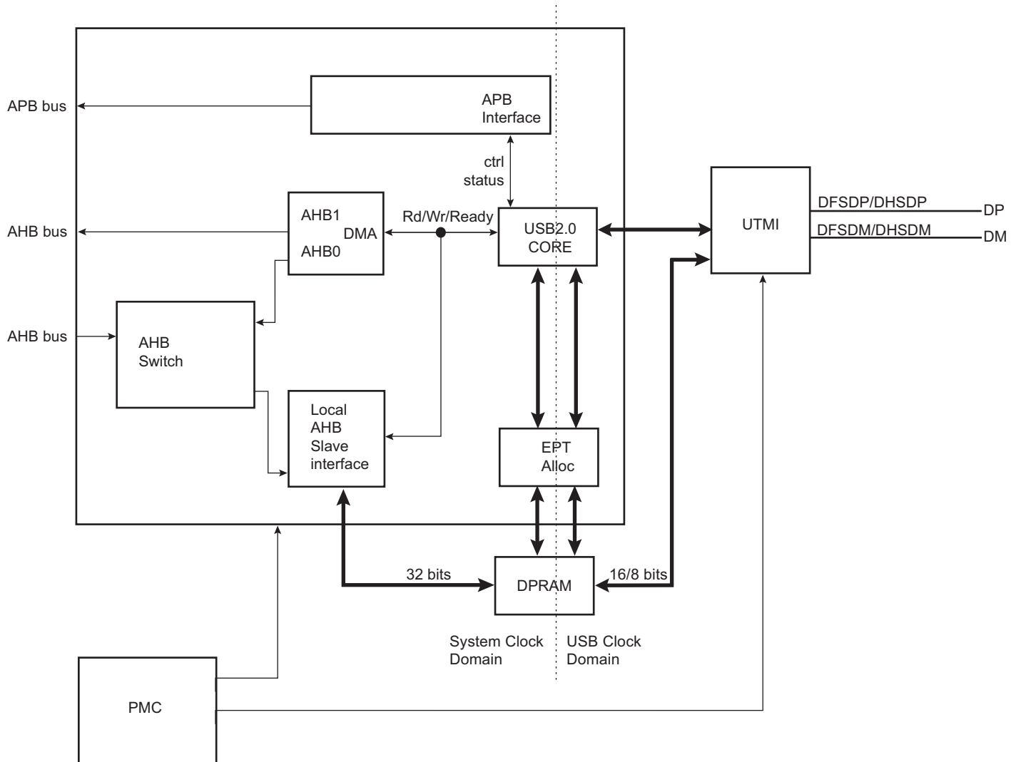
Figure 31-1: Block Diagram
