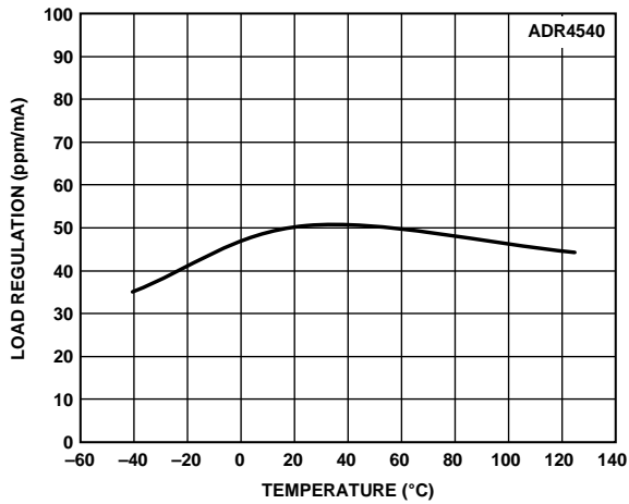
Figure 71. ADR4540 Load Regulation vs. Temperature (Sinking)
