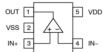
TSOP-5 (SOT23-5) and SC-88A (SC70-5) pinout
