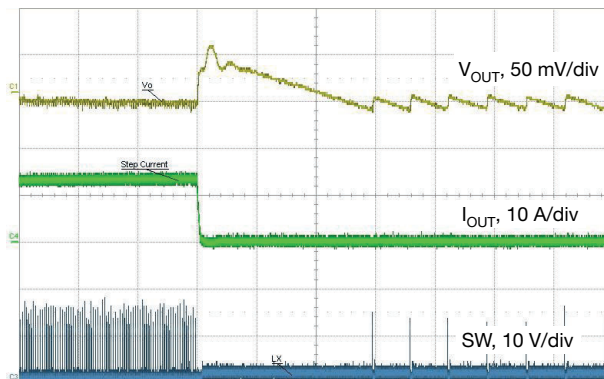
Fig. 34 - Load Release, 12 A to 0.1 A, 1 A/ \mu s, t = 50\text{ }\mu s/div Skip Mode Enabled
