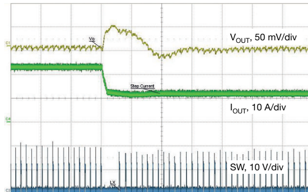
Fig. 33 - Load Release, 24 A to 12 A, 1 A/ \mu s, t = 10\text{ }\mu s/div
