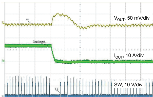
Fig. 35 - Load Release, 12 A to 0.1 A, 1 A/ \mu s, t = 20\text{ }\mu s/div Forced Continuous Conduction Mode
