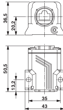
RJ45 coupling
