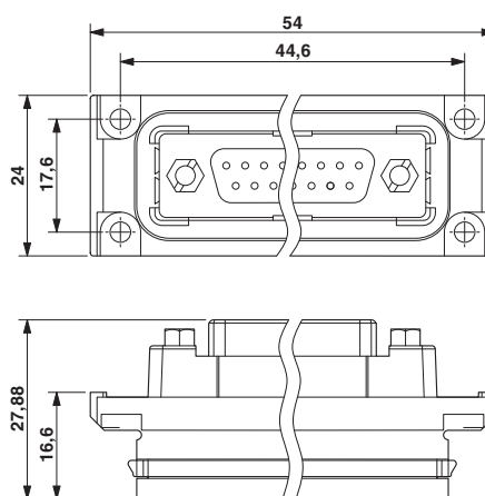
D-SUB panel mounting frame
