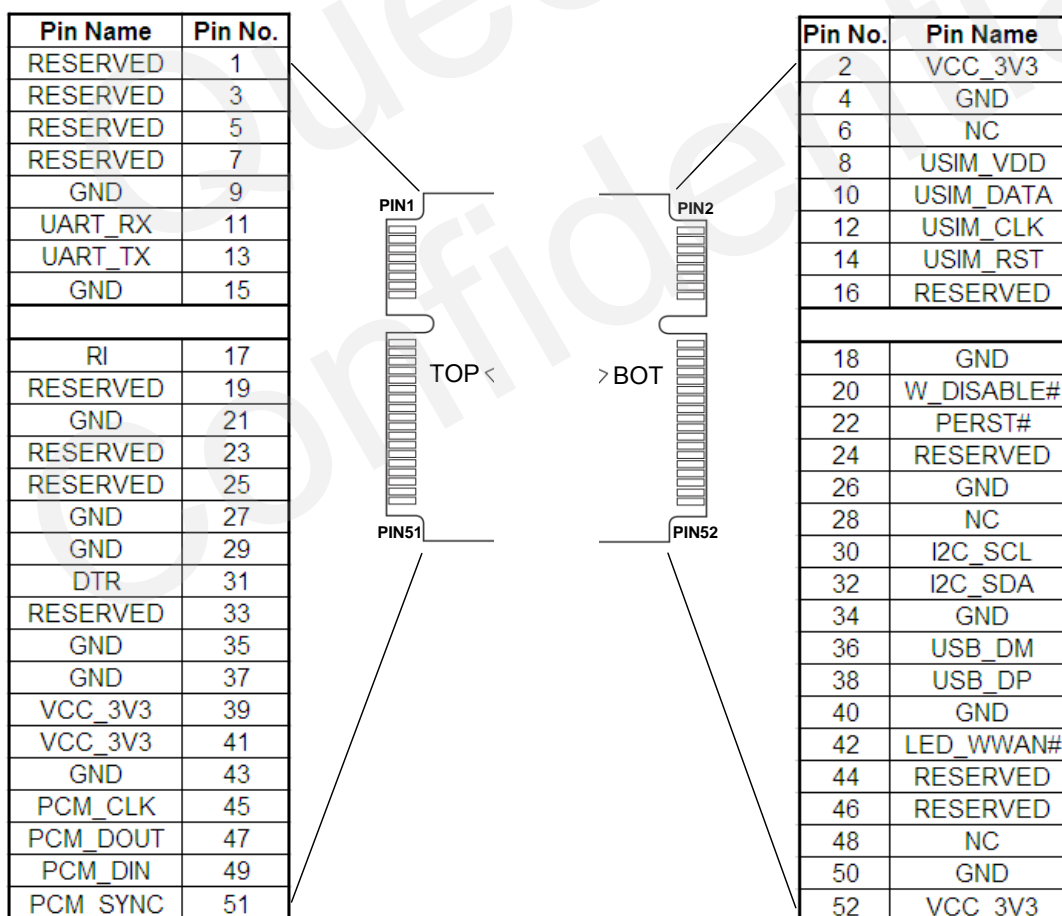
Figure 2: Pin Assignment
