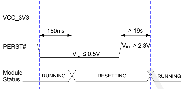
Figure 12: Timing of Resetting Module
