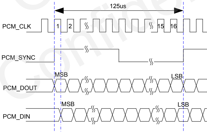
Figure 9: Timing of Auxiliary Mode
