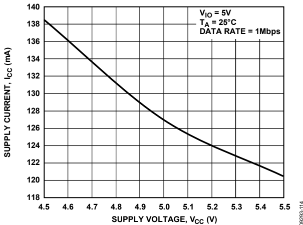
Figure 19. Supply Current, I CC vs. Supply Voltage V CC
