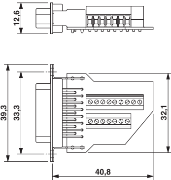
Dimensional drawing
