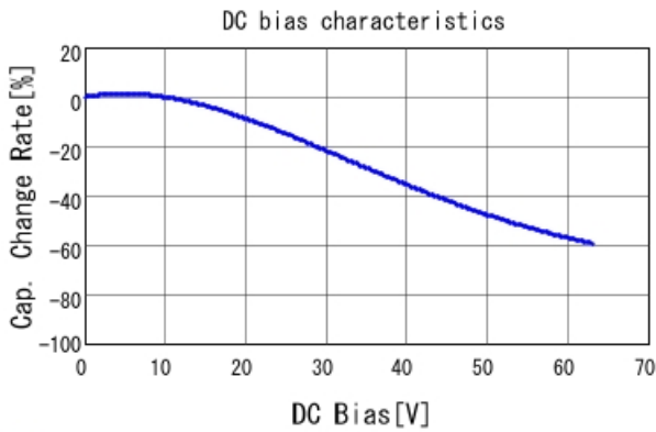
■ KCM55WR71J226MH01 C-DC bias capchange, 25.0degC, AC0.
