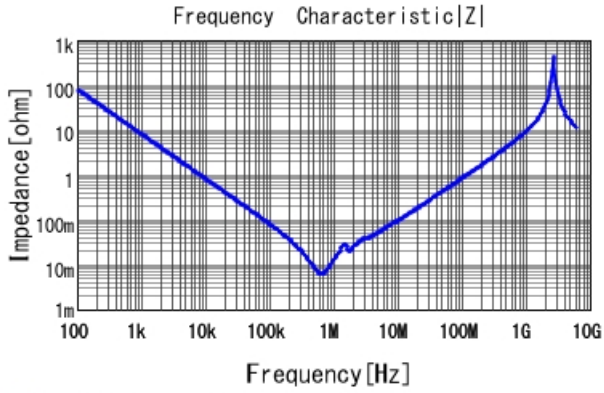
■ KCM55WR71J226MH01 |Z| DCOV, 25degC
