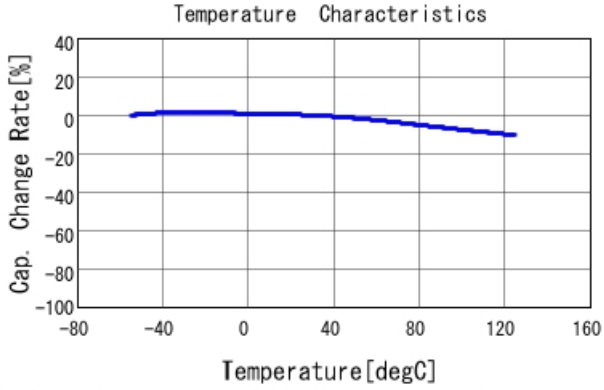
■ KCM55WR71J226MH01 C-Temp. capchange, DCOV, ACO. 5Vrms
