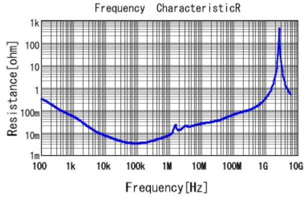
■ KCM55WR71J226MH01 R DCOV, 25degC
