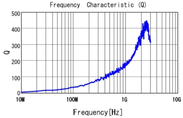
■ LQP03HQ0N6W02 Q
