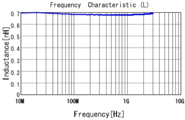
■ LQP03HQ0N6W02 L
