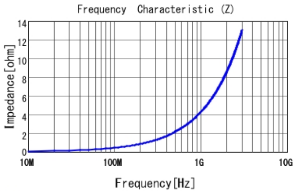
■ LQP03HQ0N6W02 |Z|
