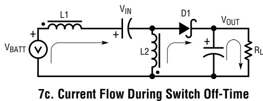
Figure 7. SEPIC Topology and Current Flow
