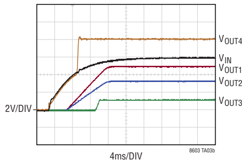
Start-Up Sequence
