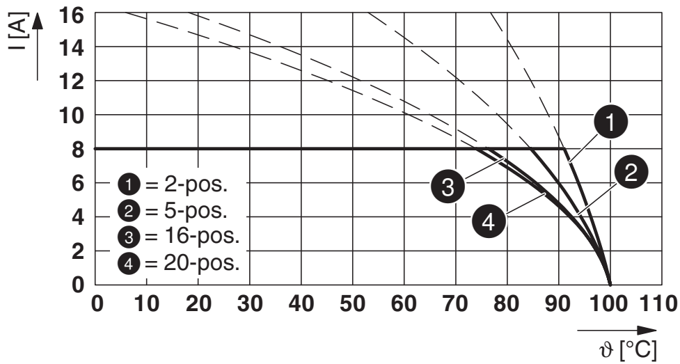
Type: FK-MCP 1,5/...-ST-3,5 with MCV 1,5/...-G-3,5
