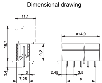
Type: MC 1,5/...-ST-3,5 with MCV 1,5/...-G-3,5
