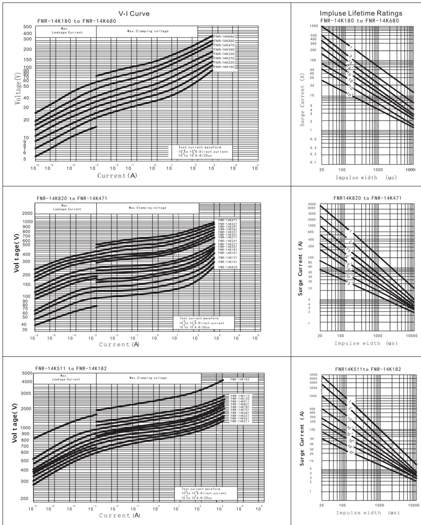
*14K 系列 V-I 特性曲线和最大浪涌电流降额曲线 14K Series V-I Curve and Max. Surge Current Derating Curves
