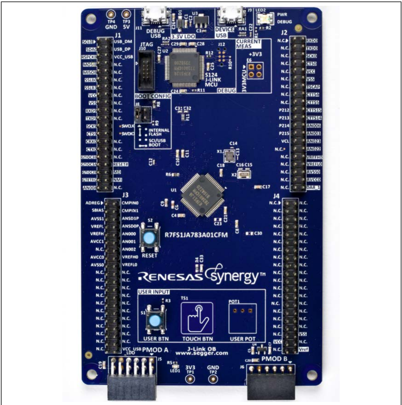
Figure 1 TB-S1JA Board
