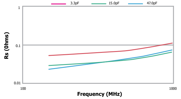
ESR vs. Frequency DLI C06 UL Series
