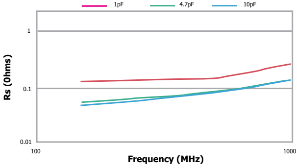
ESR vs. Frequency DLI C04 UL Series
