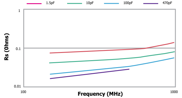
ESR vs. Frequency DLI C17 UL Series
