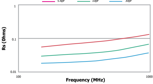
ESR vs. Frequency DLI C07 UL Series
