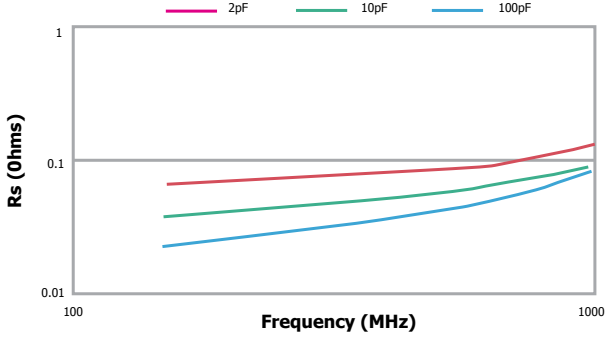
ESR vs. Frequency DLI C11 UL Series
