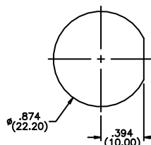
Mounting Holes
