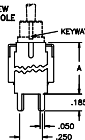
SIDE VIEW - SINGLE AND DOUBLE POLE
