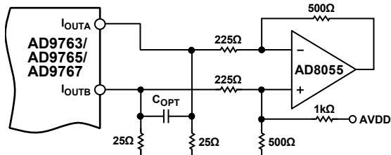
Figure 74. Single-Supply DC Differential-Coupled Circuit
