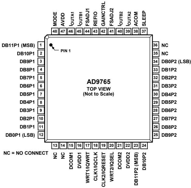
Figure 4. AD9765 Pin Configuration
