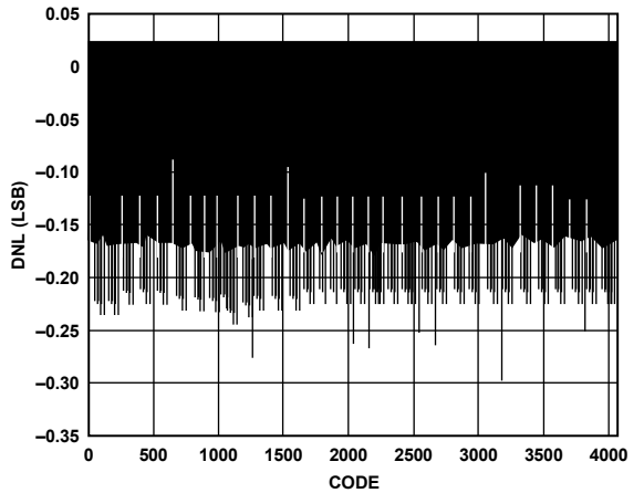
Figure 34. Typical DNL
