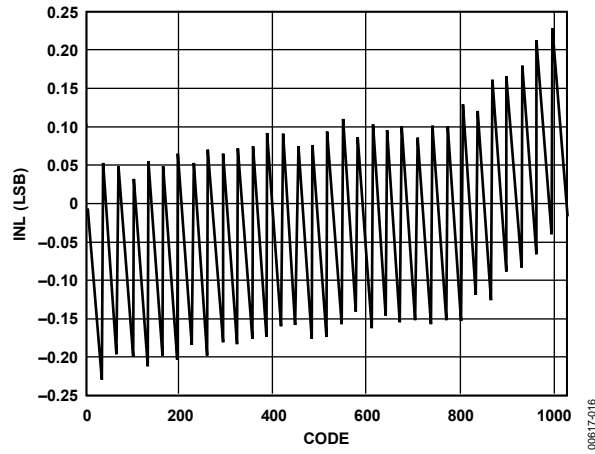
Figure 16. Typical INL
