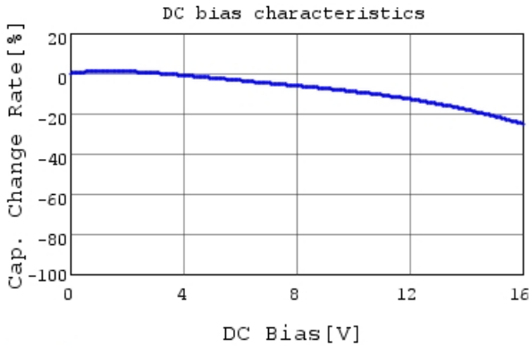
GRM155R71C153KA01 C-DC bias capchange, 25.0c
