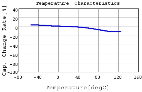
GRM155R71C153KA01 C-Temp. capchange, DC0.0V,
