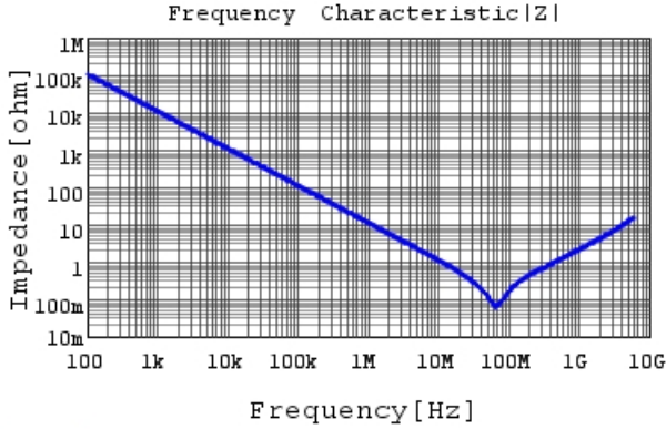
GRM155R71C153KA01 |Z| DCOV,25degC
