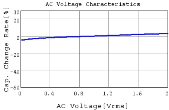
GRM155R71C153KA01 C-AC Voltage capchange, DC
