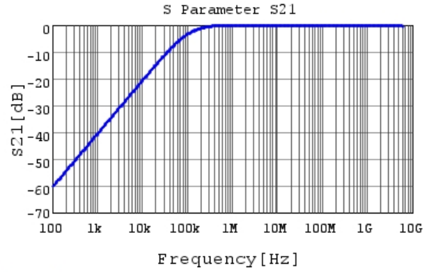
GRM155R71C153KA01 S21 DC0V,25degC
