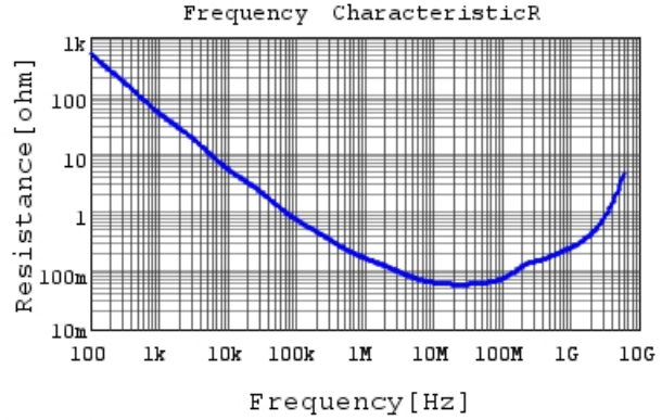
GRM155R71C153KA01 R DCOV,25degC
