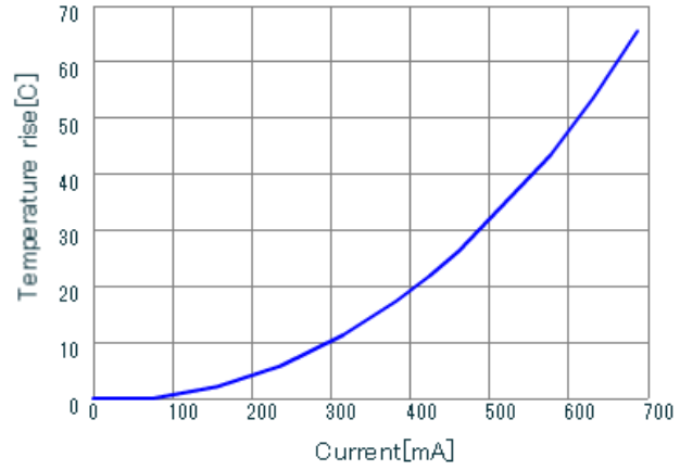
LQH44PN470MJ0 DT_Current
