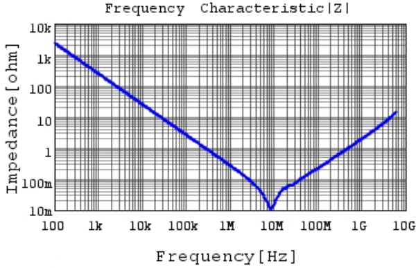
GCM188R71E105KA64 |Z| DC0V, 25degC
