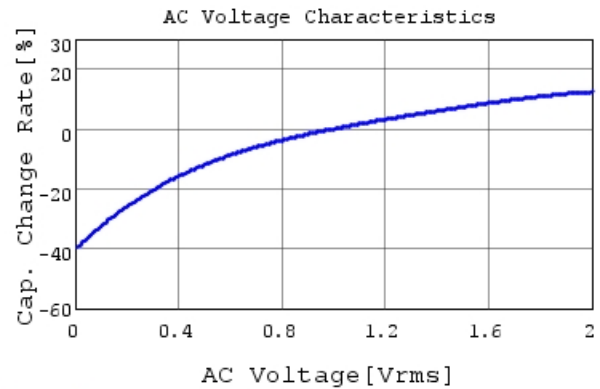
GCM188R71E105KA64 C-AC Voltage capchange, DC
