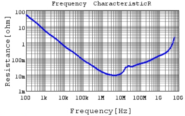
GCM188R71E105KA64 R DC0V, 25degC
