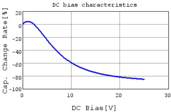
GCM188R71E105KA64 C-DC bias capchange, 25.0c
