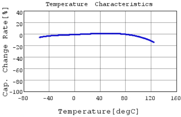
GCM188R71E105KA64 C-Temp. capchange, DC0.0V,
