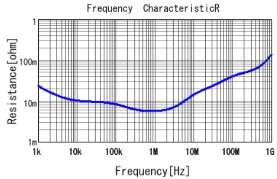
■ ECASD41A107M040KA0 R DCOV, 25degC
