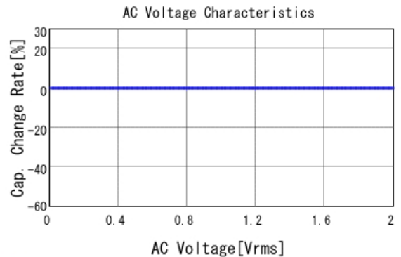
■ ECASD41A107M040KA0 C-AC Voltage capchange, DCOV, 25.0
