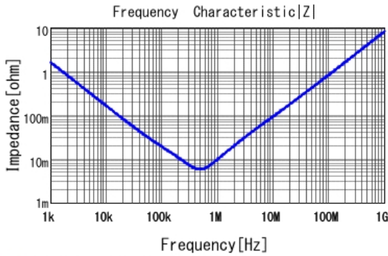
■ ECASD41A107M040KA0 |Z| DCOV, 25degC
