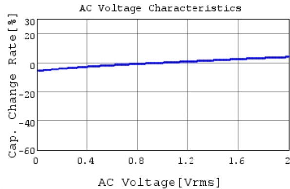
GCM155R71H104KE02 C-AC Voltage capchange, DC
