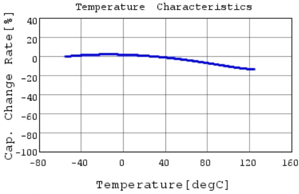
GCM155R71H104KE02 C-Temp. capchange, DC0.0V,
