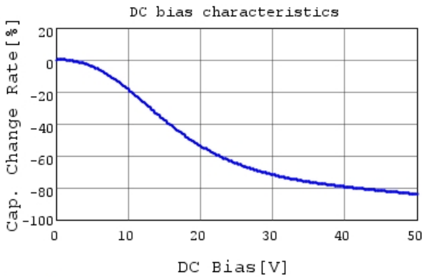
GCM155R71H104KE02 C-DC bias capchange, 25.0c
