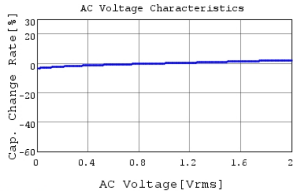
GCM155R71H102KA37 C-AC Voltage capchange, DC
