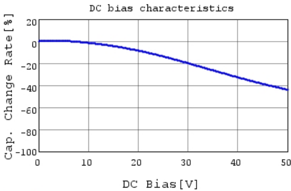
GCM155R71H102KA37 C-DC bias capchange, 25.0c
