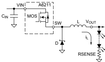
Figure 7: Simplified Buck Controller Equations, and Reference Circuit and Waveforms
