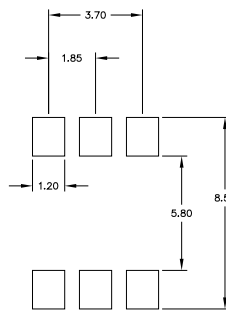
SUGGESTED LAND PATTERN
