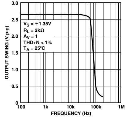
TPC 30. Maximum Output Swing vs. Frequency at 2.7\text{ V}
