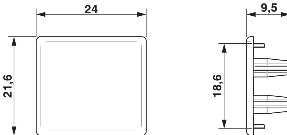
Dimensional drawing
