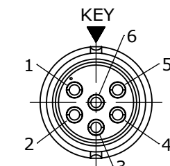
WIRING END W6282-6SG-P-5XX
