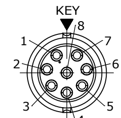
WIRING END W6282-8SG-P-5XX
