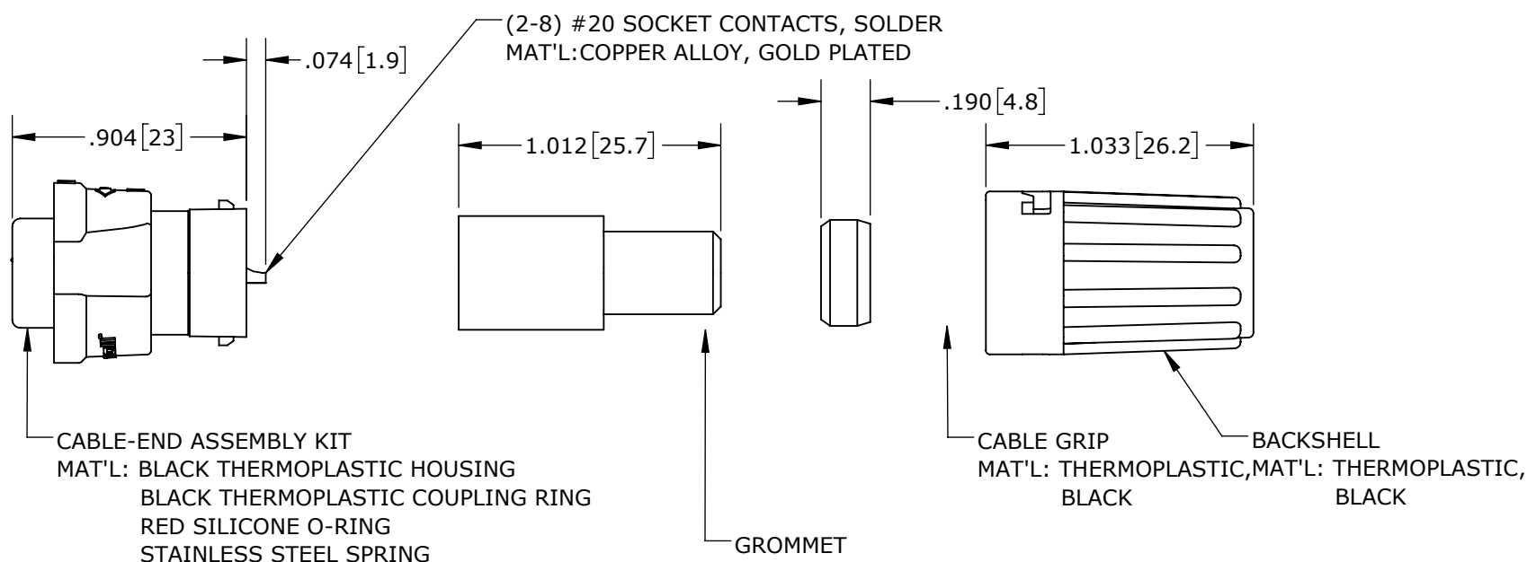
SHOWN ASSEMBLED KIT ASSY: W6282-2SG-P-5XX SHOWN
