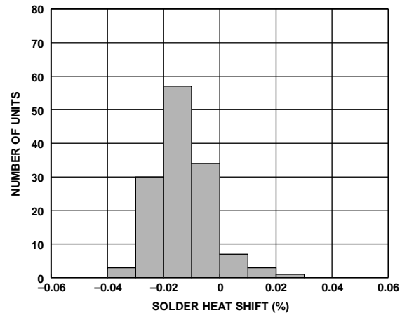
Figure 101. ADR4550 Solder Heat Resistance Shift (3 x Reflow)
