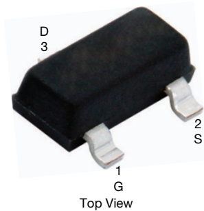
SOT-23 (TO-236)
