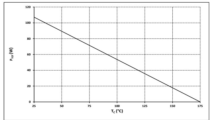
Figure 4 Power Derating
