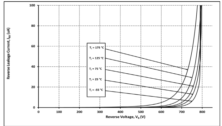
Figure 2 Reverse Characteristics
