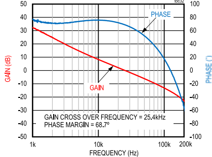
BODE PLOT FIGURE 5 CIRCUIT
