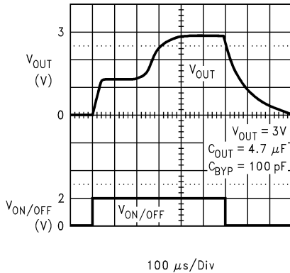
Figure 7-13. Turnon Waveform (Legacy chip)
