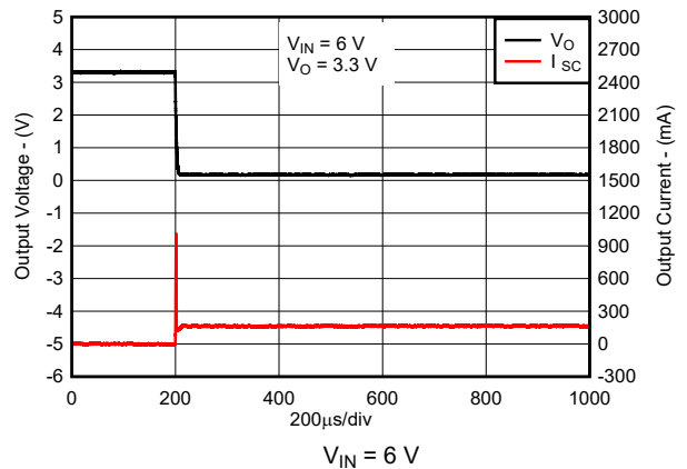
Figure 5-30. Short-Circuit Current versus Time (New Chip)
