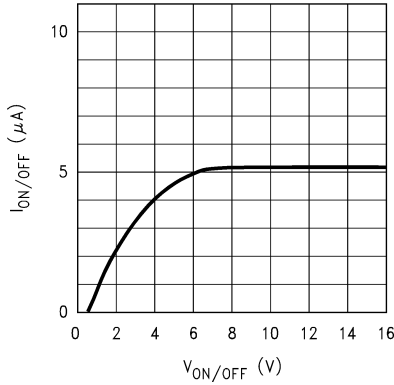
Figure 5-37. ON/ \overline{\text{OFF}} Pin Current versus V_{\text{ON/OFF}} (Legacy chip)
